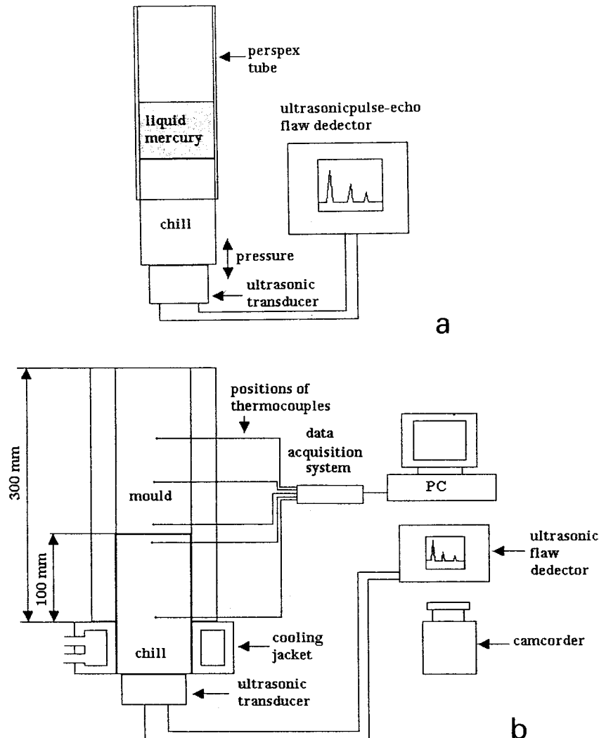
Figure 1 Experimental apparatus used to investigate the ultrasonic reflection from the casting-chill interface. (a) For the experiment with liquid Hg cast onto a Cu chill. (b) For the experiment with Al-4.5 wt%Cu alloy cast onto a Cu chill.
