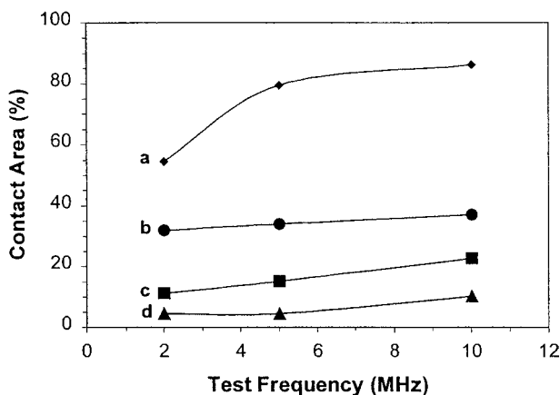
Figure 3 Variation in estimated contact area for liquid Hg cast onto a Cu chill with varying chill surface finish, for three different test frequencies. a—4000, b—2500, c—400 and d—280 grade emery papers. (Pouring height of 28 cm from chill surface.)
